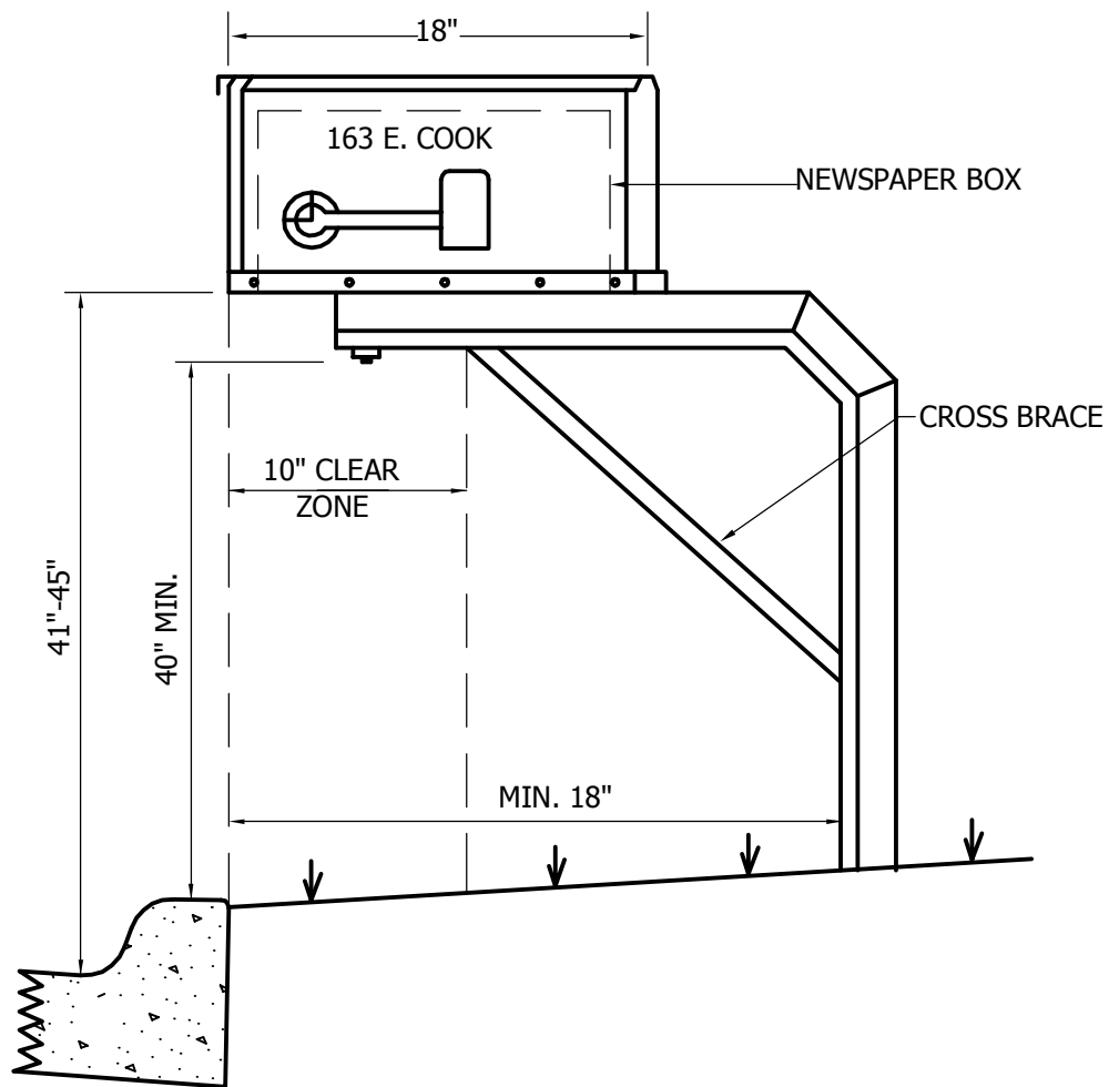
SIDE VIEW
